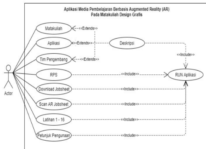
Fig. 4. Use case Diagram of AR Media
